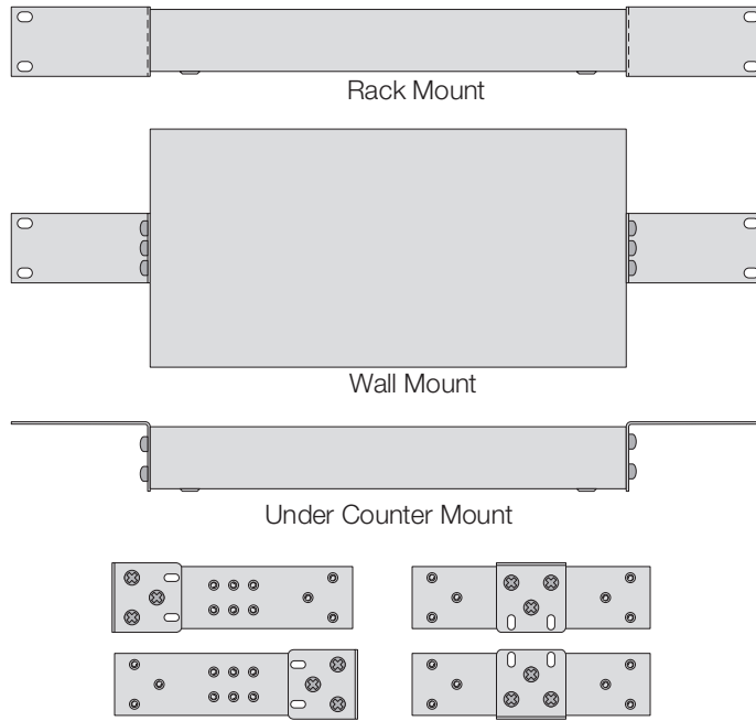
Mounting brackets can be installed front, rear, up, or down
