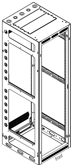
The rack includes a rear door and top closure panels (rear door can be omitted if not needed, see ordering option, pg. 2). A front door is optional, order separately.
