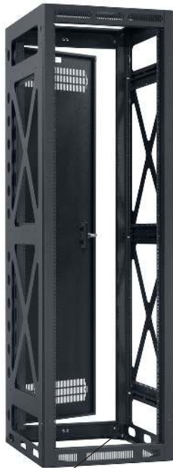
Corner weldments with holes for anchors (by others)
