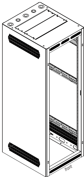
The rack includes a rear door and top closure panels (rear door can be omitted if not needed, see ordering option, pg. 2). A front door is optional, order separately.
