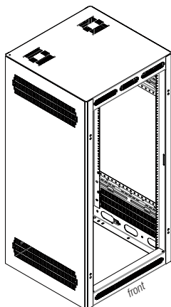
The rack includes a rear door (rear door can be omitted if not needed, see ordering option, pg. 2). A front door is optional, order separately.
