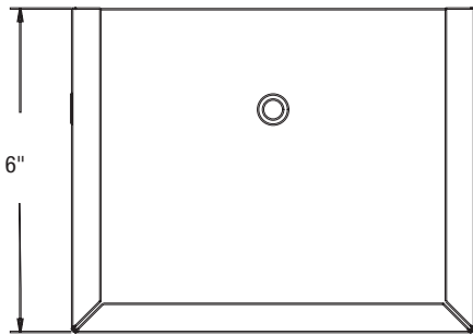
Knockouts on four sides (1/2"-3/4")
