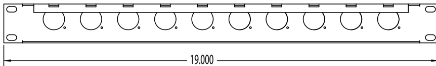
REAR VIEW
