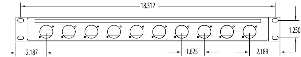
FRONT VIEW
